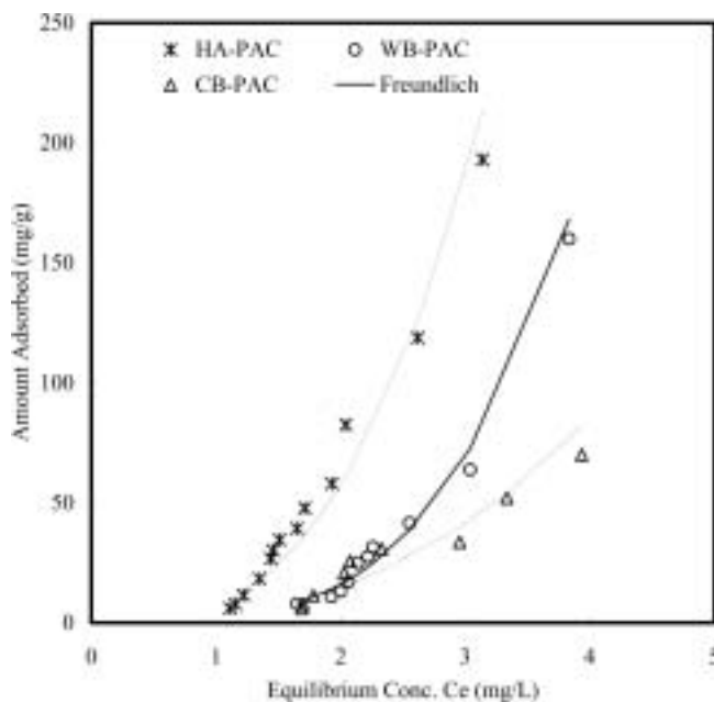
Fig. 3. Adsorption isotherm for the three PACs (equilibrium time 4 days, temperature 25 °C, average initial TOC concentration 4.6 mg/L, isotherm constants - WB PAC: k=1.3097 , n=0.2769 , Error % = 13.61; CB PAC: k=2.606 , n=0.3973 , Error % = 25; CB PAC: k=7.577 , n=0.3429 , Error % = 25.22).
